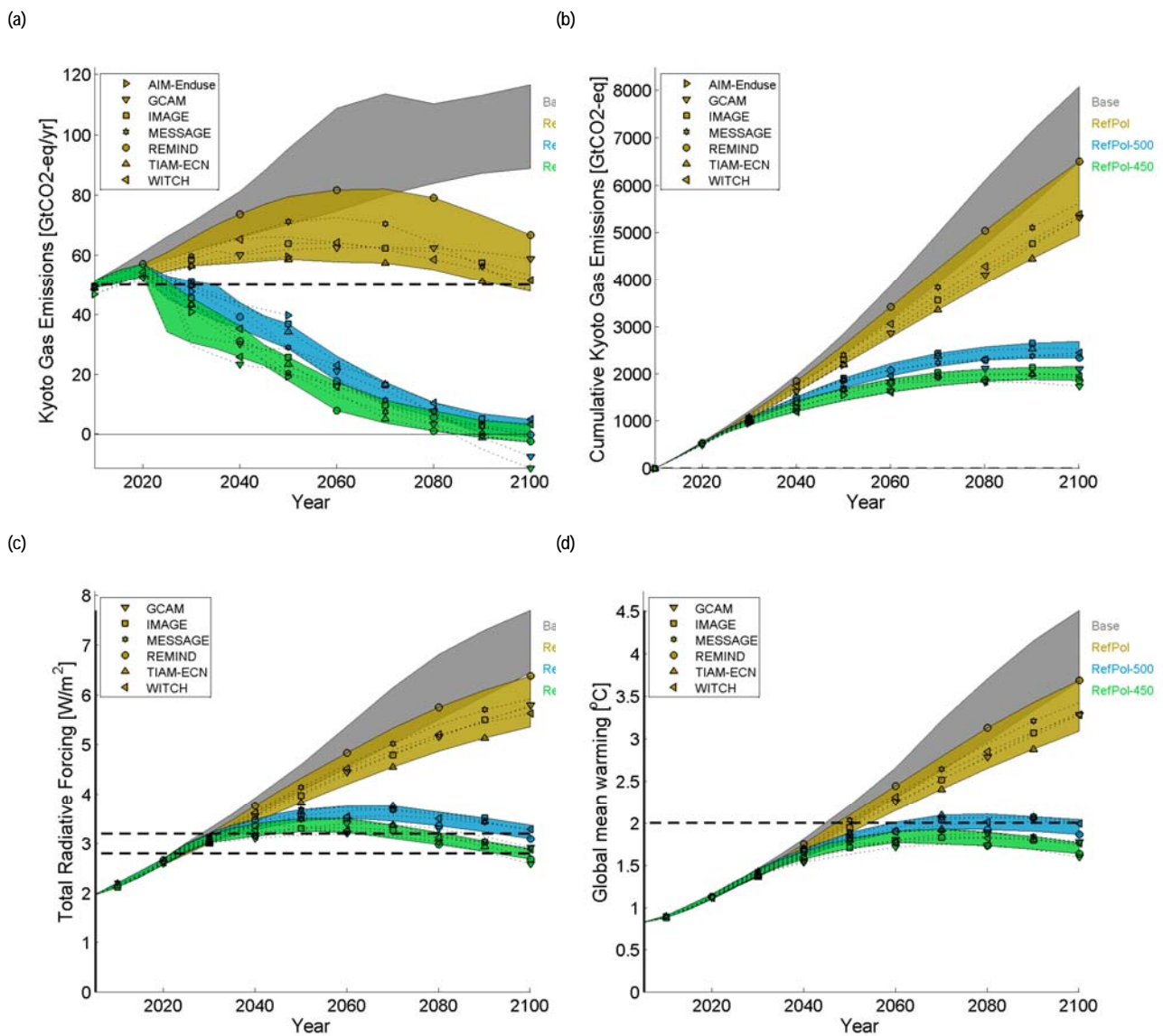
Figure 1: CO 2 equivalent Kyoto gas emissions over the period 2010-2100 per year (Panel a) and in cumulative terms (Panel b) for a subset of LIMITS scenarios (see Figure S1 for corresponding StrPol scenarios). The resulting median radiative forcing and global mean warming as calculated with MAGICC are shown in Panel c & d. The AIM and GCAM models were not included in the funnels because AIM projected emissions only out to 2050 and GCAM showed a qualitatively different behavior due to a strong afforestation and negative emissions response to the adoption of the long term target.
