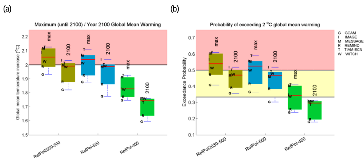
Figure 6: Median global mean warming (panel a) and probability of exceeding 2°C for the Durban Platform Scenarios (panel b). The left (higher) bars show the maximum warming / exceedance probability in the 21 st century; the right (lower) bars shows the warming / exceedance probability in 2100.
