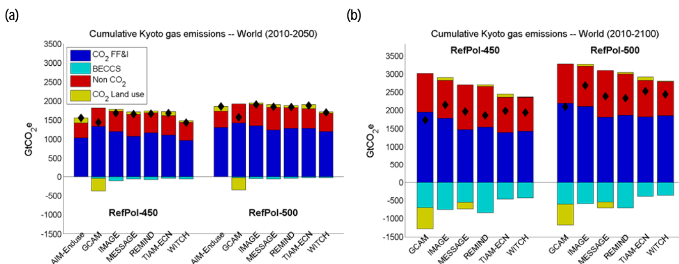
Figure 4: Cumulative Kyoto gas emissions over the period 2010-2050 (a) and 2010-2100 (b) broken out into individual sectors. The black diamond shows net total cumulative emissions.
