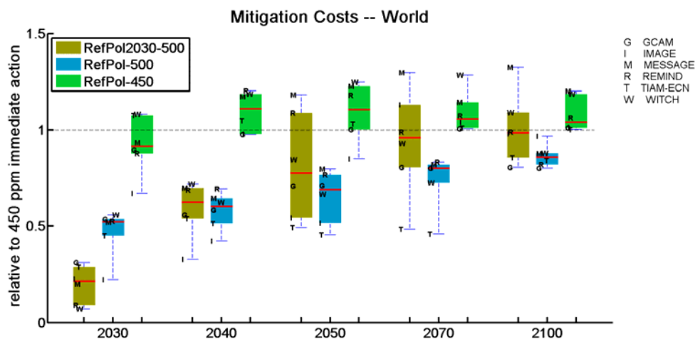
Figure 7: Mitigation costs over time for the Durban Platform scenarios with lenient reference policy and the “delay until 2030” scenario. Shown are (a) consumption losses as a fraction of baseline consumption as projected in general equilibrium models (MESSAGE, REMIND, WITCH), (b) abatement costs measured in terms of the area under the MAC (IMAGE, GCAM) or total additional energy system costs (TIAM-ECN) as a fraction of baseline output, and (c) mitigation costs relative to the 450 ppm immediate action scenario. A value of one indicates identical costs at the given point in time between the given and the 450 ppm scenario.
