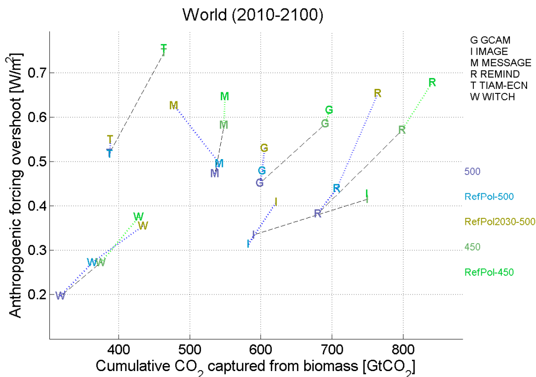
Figure 6: Radiative forcing overshoot (of Year 2100) forcing vs. cumulative negative emissions from BECCS.
