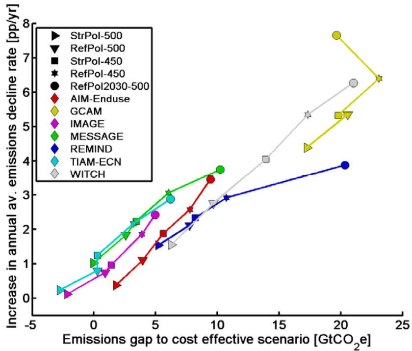
Figure 3: Emissions gap in the year of target adoption vs. the increase in annual average emissions decline rate between the decades before and after target adoption.
