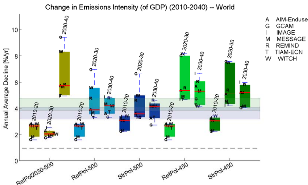
Figure 2: Annual average emissions intensity decline rate (of Kyoto gases per unit of GDP) for the periods 2010-20 (left bars), 2020-30 (middle bars) and 2030-40 (right bars). The dashed line shows the average decline rate over the period 2005-2010 (from EDGAR, 2011, and the assumption of 11% growth in GWP), and the shaded areas the range of decline rates projected by the models (excluding GCAM due to the afforestation dynamics) for immediate action on 500 ppm (lower area) and 450 ppm CO 2 e (upper area).
